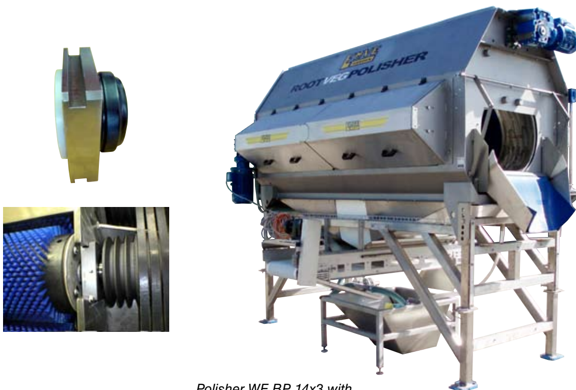
Polisher WE BP 14x3 with filterconveyor and tank
